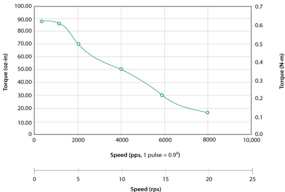
4418L-36 24VDC, 2.0 Amps/Phase, Bipolar, 1/2 Stepping
